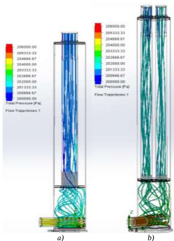
Fig. 2. Flow trajectories and total pressure values: a – Commercial, b – New Design
